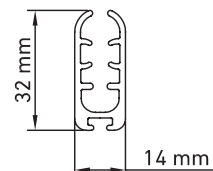
Terminal Plano Flat Bottom Weight Lame finale Plate
