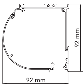
Saxun Box 92 curvo Curved Saxun Box 92 Saxun Box 92 courbe
