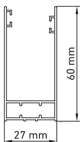
Guía 60x27 60x27 Guide Coulisse 60x27
