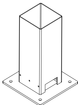
Fixing surface 304 stainless steel column base Code 050214
