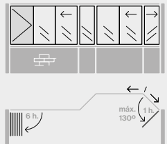
Four-sided terrace with opening on both sides. 135° pass-angle
