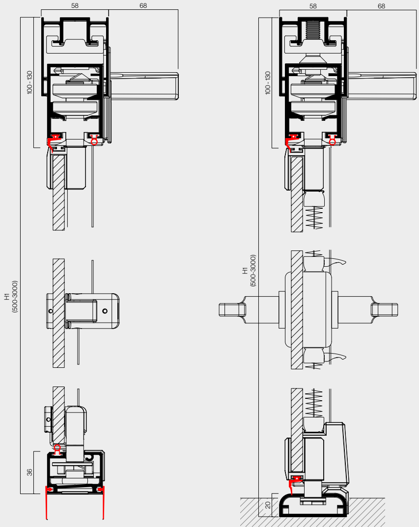
Azur normal rail Azur passable rail
