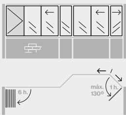
Four-sided terrace with opening on both sides. 135° angle pass-through
