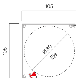
Box 105 profile Wind Screen V.2 024969
